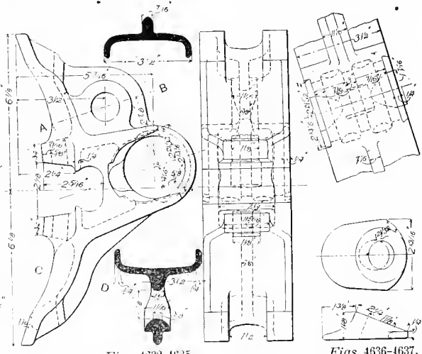
CHRISTIE BRAKE-HEAD FOR UNIVERSAL BRAKE-BEAM.
